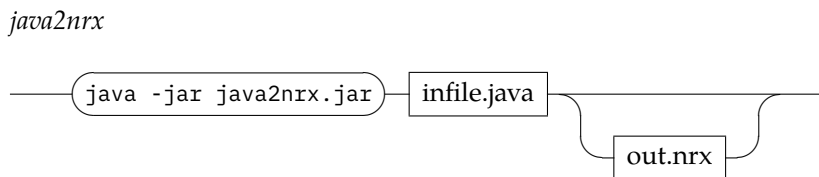
FIGURE 2: Java2nrx 1
